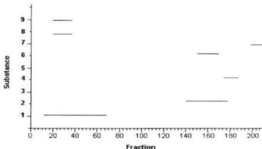
FIGURE 3: Fractions collected after separation by DCCC showing the separation of substances 1, 2, 6, 7, 8 and 9 using solvent system (II) \text{CHCl}_3 :MeOH: \text{H}_2\text{O} 13:7:4 v.v.v. descending mode.
