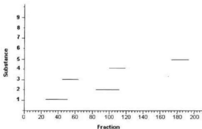
FIGURE 2: Fractions collected after separation by DCCC showing the separation of substances 1-5 using solvent system (I) \text{CHCl}_3 :MeOH: \text{H}_2\text{O} , 43:37:20 v.v.v. descending mode.
