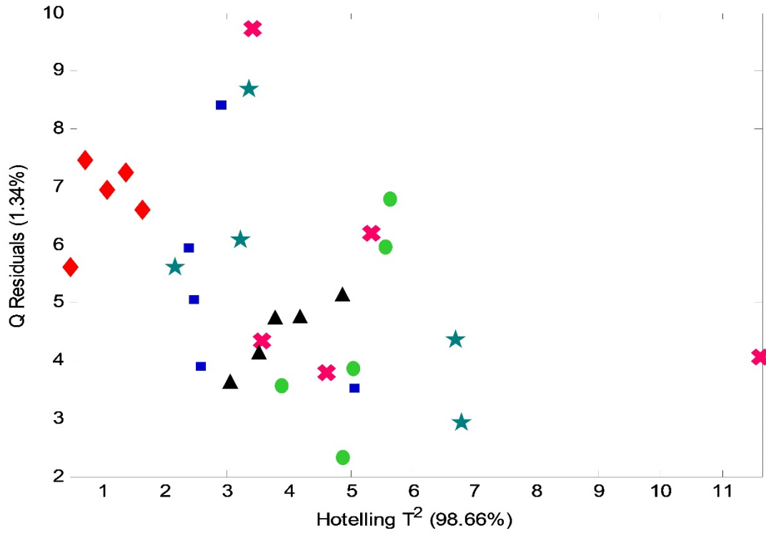
Figure 1S. Q residuals (1.34%) versus Hotelling's T 2 (98.66%) plot of the PCA. Ps (black triangles), PsBRSPC (red diamonds), Pa (blue squares), PaBRSMC (blue stars), Pc (pink crosses), and PcBRSSF (green dots).
