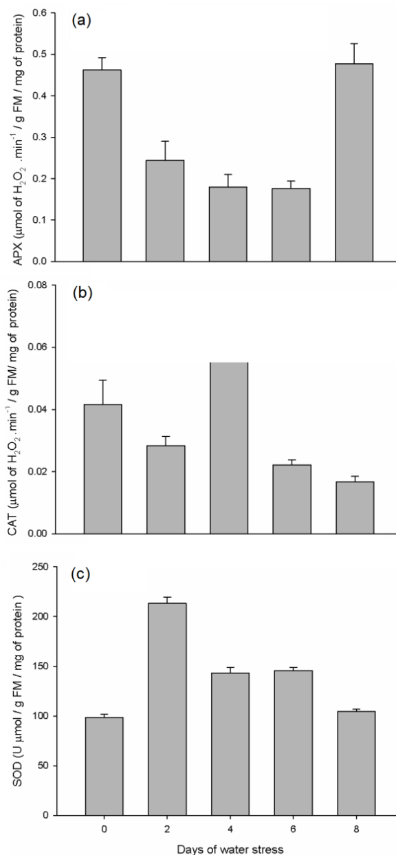
Figure 1. Activity of the enzymes ascorbate peroxidase-APX (a), catalase-CAT (b) and superoxide dismutase-SOD (c), in Piper aduncum grown under 0, 2, 4, 6, and 8 days of water suppression.
