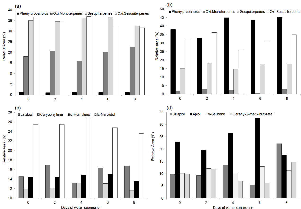
Figure 2. Classes of constituents of the essential oil of the leaves (a), roots (b) and major compounds of the leaves (c) and roots (d) of Piper aduncum grown under water suppression (0, 2, 4, 6, and 8 suppression days).
